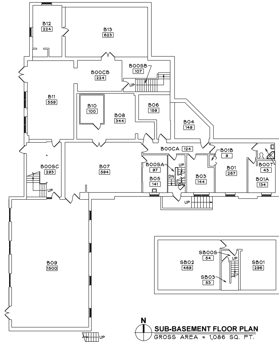
BASEMENT FLOOR PLAN GROSS AREA = 6,940 SQ. FT.
