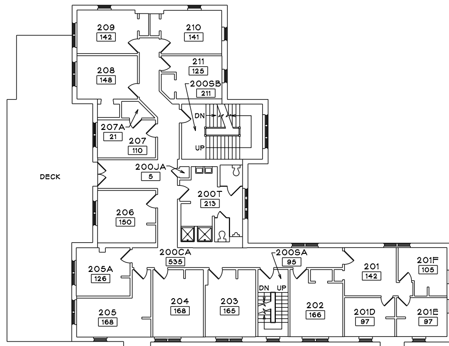
N SECOND FLOOR PLAN GROSS AREA = 3,774 SQ. FT.
